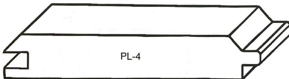
PL-4 3/4" x 4 5/16" PLANKING
