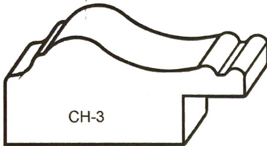
CH-3 1 1/8" x 2 1/2" CHAIR RAIL
